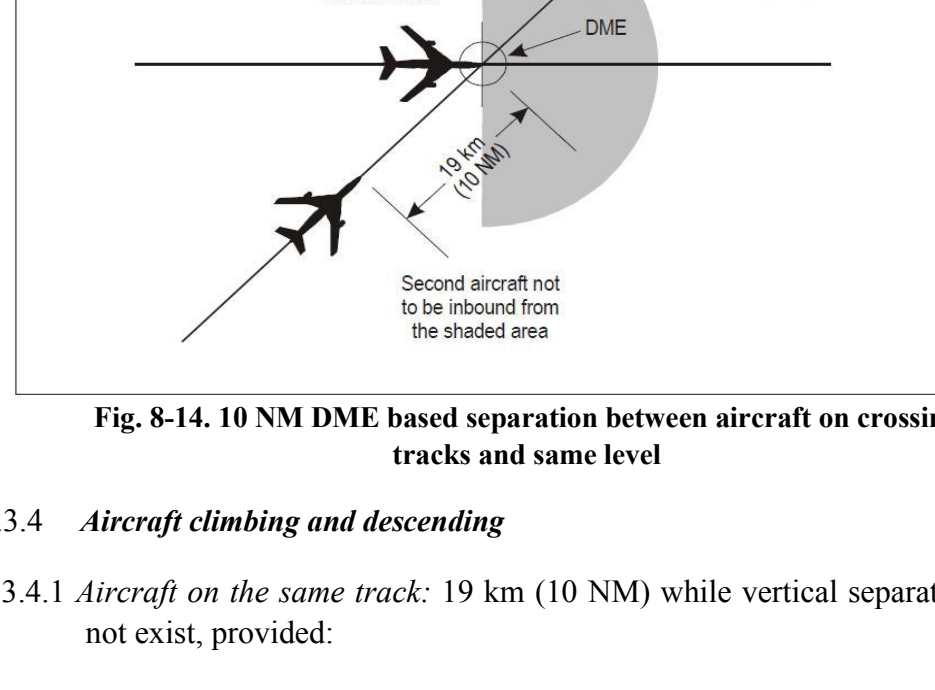
Fig. 8-14. 10 NM DME based separation between aircraft on crossing tracks and same level
