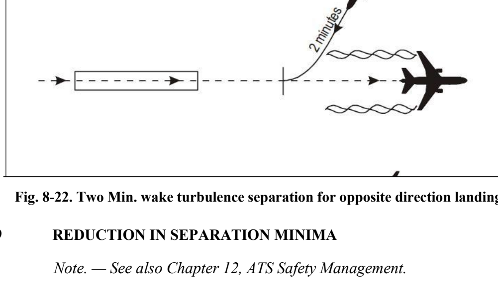
Fig. 8-22. Two Min. wake turbulence separation for opposite direction landing
