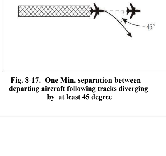
Fig. 8-17. One Min. separation between departing aircraft following tracks diverging by at least 45 degree
