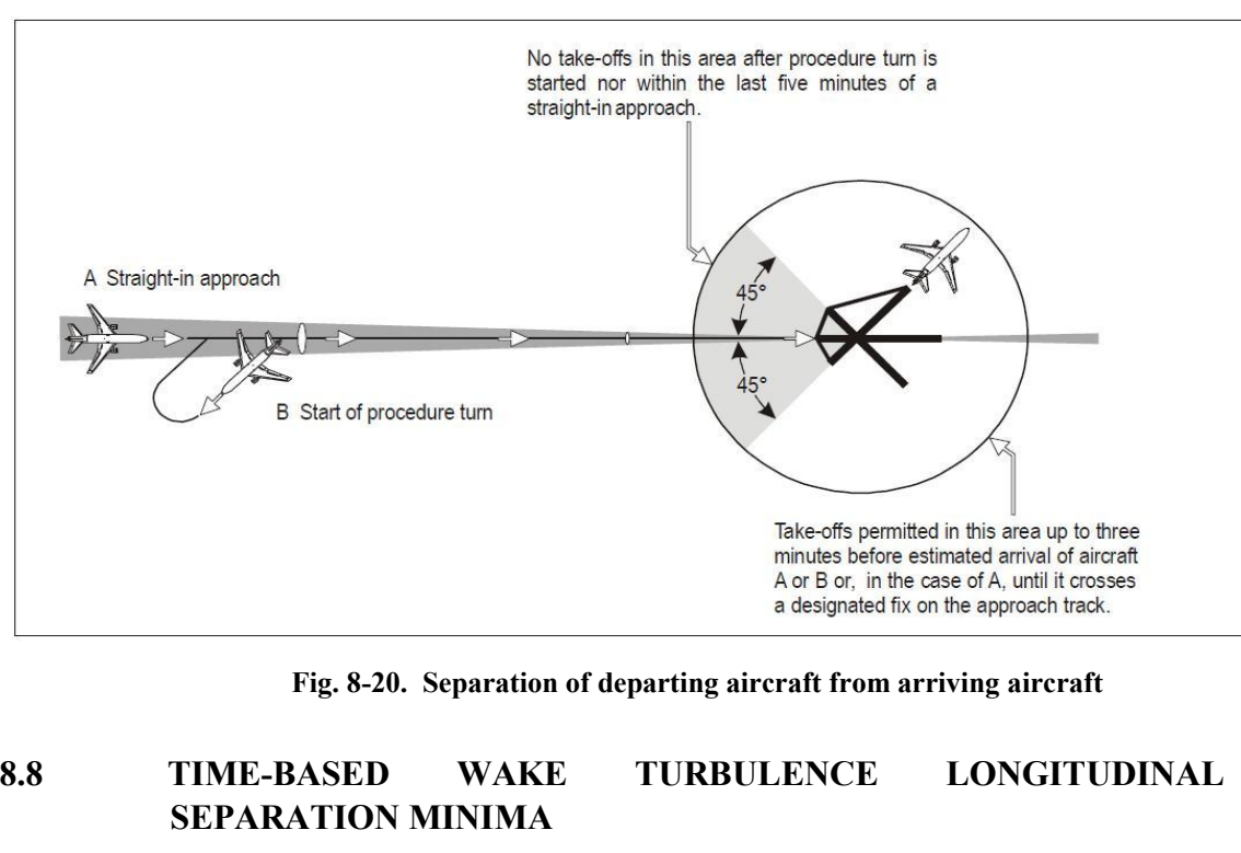
Fig. 8-20. Separation of departing aircraft from arriving aircraft
