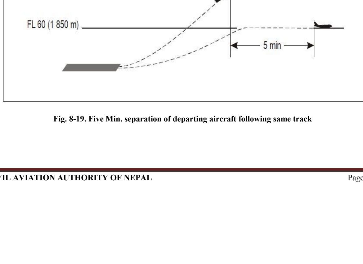
Fig. 8-19. Five Min. separation of departing aircraft following same track
