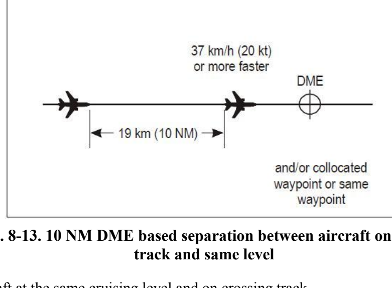
Fig. 8-13. 10 NM DME based separation between aircraft on same track and same level
