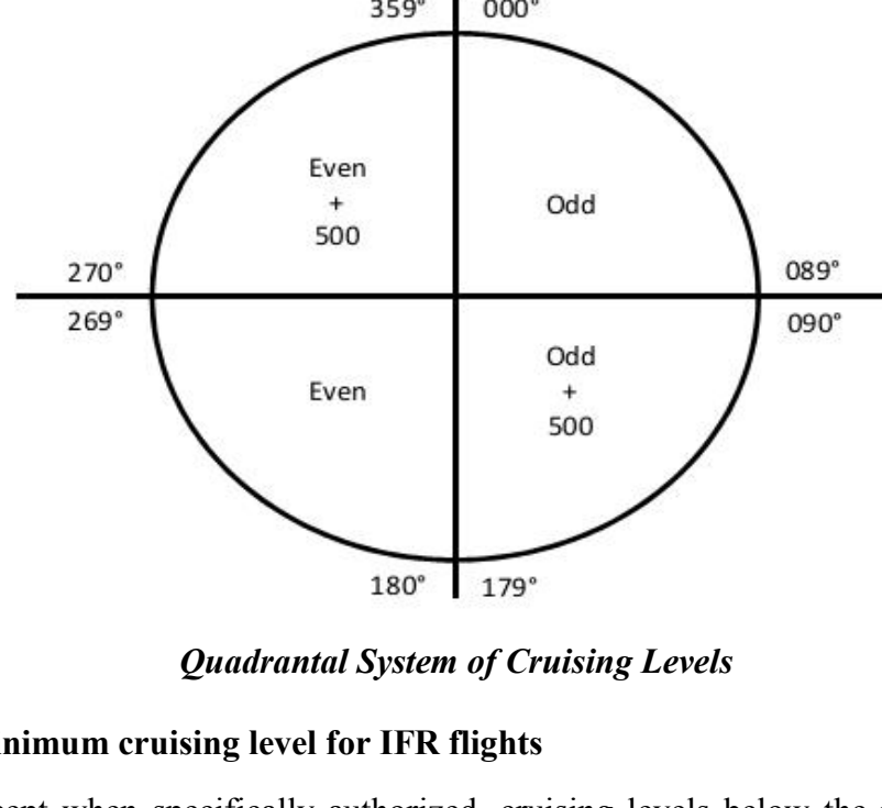
Quadrantal System of Cruising Levels
